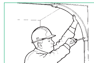
3. Position the Plaster Arch in the partition corner and screw to timber studding. Taking care to align the arch. Do not over-tighten screws.
