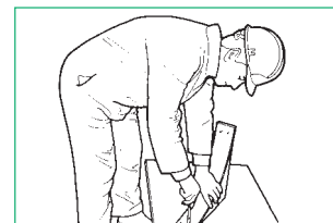
2. Insert No. 8 plated wood screws or plasterboard screws into the Plaster Arch (30mm length). Centre line of arch to align with centre of stud.
