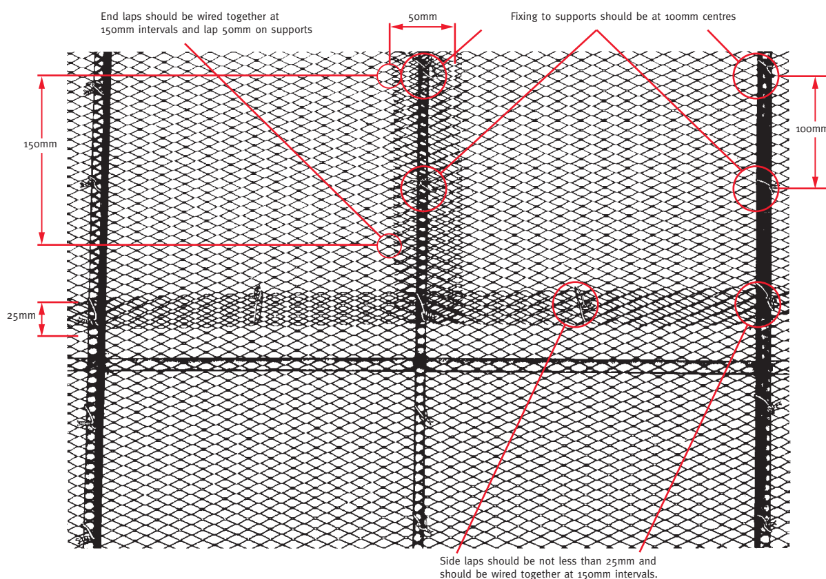
Fig. 4 General fixing information for fixing to metal/timber supports.
