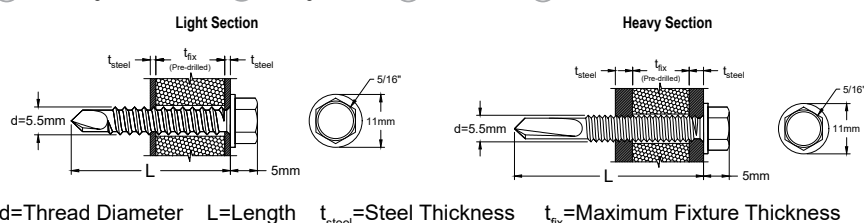
LIGHT SECTION
